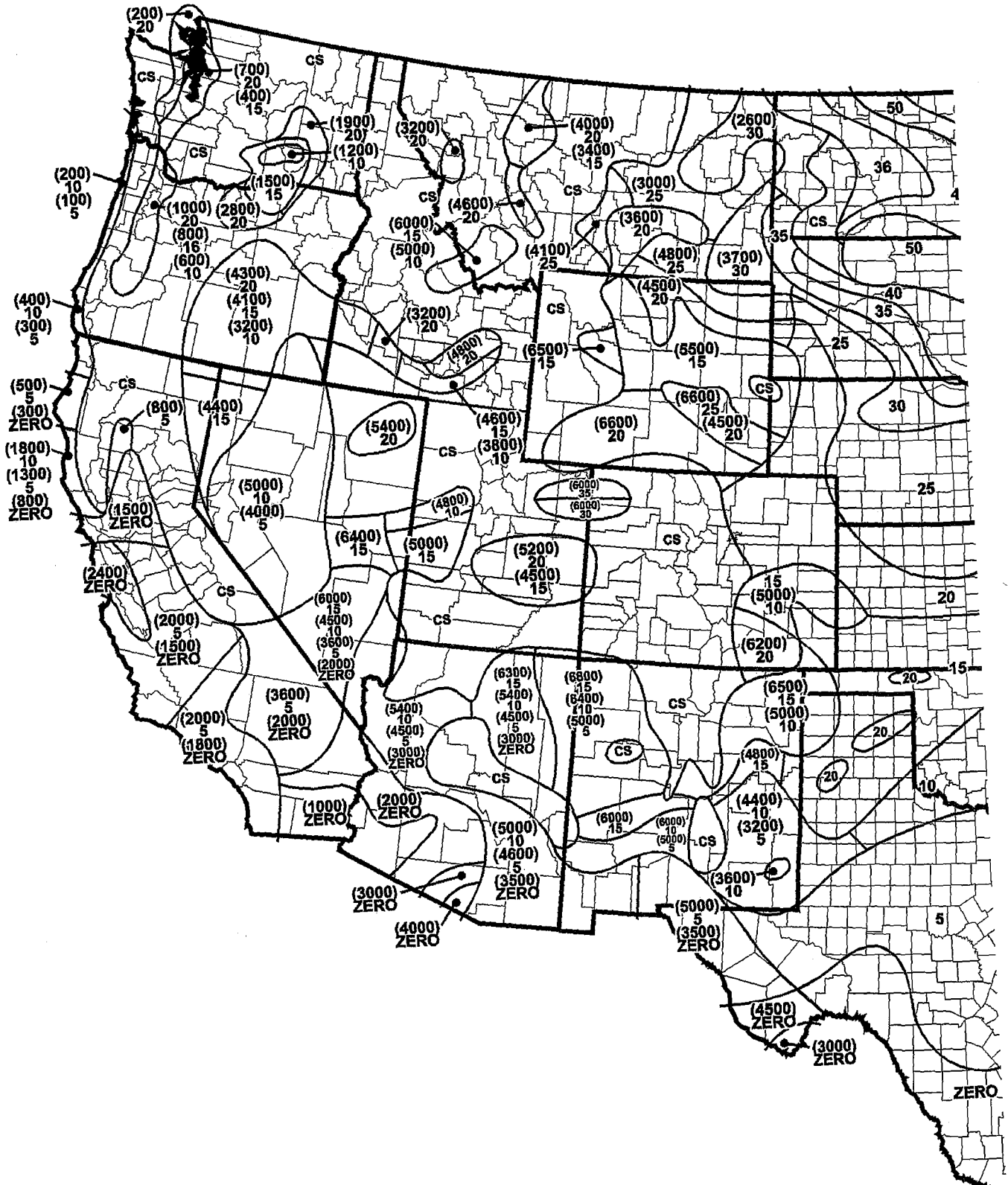
FIGURE 1608.2 GROUND SNOW LOADS, p_g , FOR THE UNITED STATES (psf)
