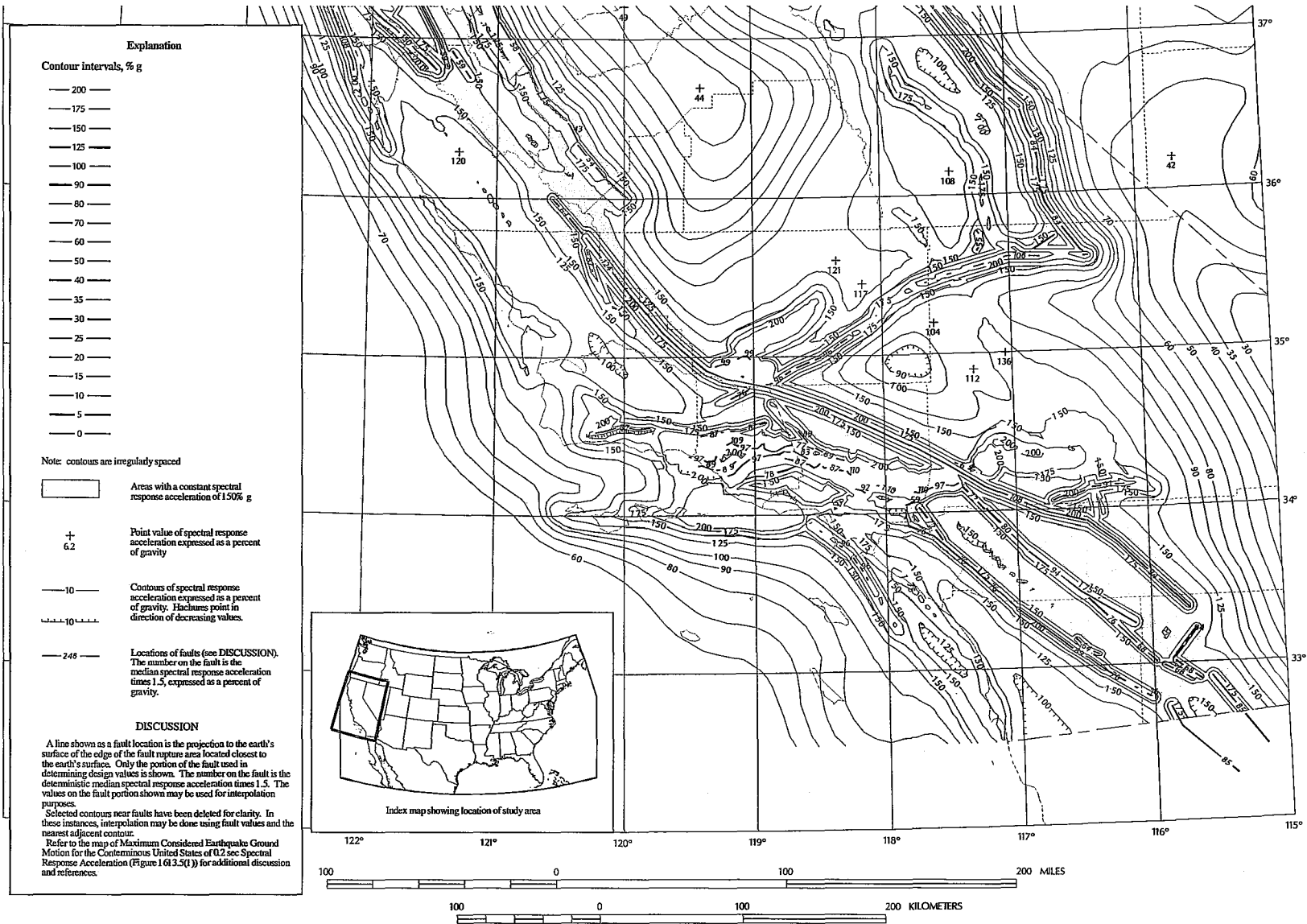
FIGURE 1613.5(3)—continued MAXIMUM CONSIDERED EARTHQUAKE GROUND MOTION FOR REGION 1 OF 0.2 SEC SPECTRAL RESPONSE ACCELERATION (5% OF CRITICAL DAMPING), SITE CLASS B
