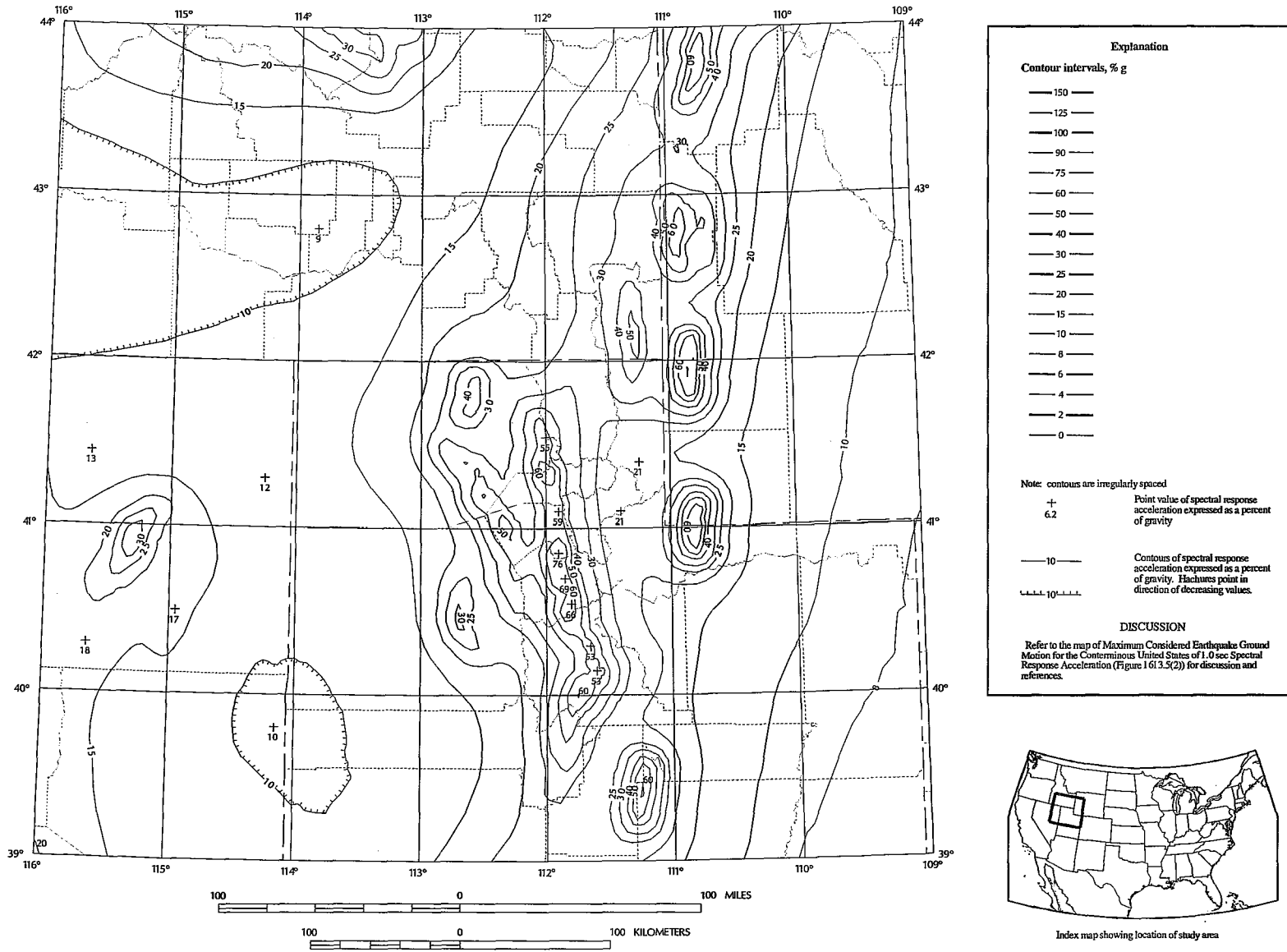
FIGURE 1613.5(6) MAXIMUM CONSIDERED EARTHQUAKE GROUND MOTION FOR REGION 2 OF 1.0 SEC SPECTRAL RESPONSE ACCELERATION (5% OF CRITICAL DAMPING), SITE CLASS B
