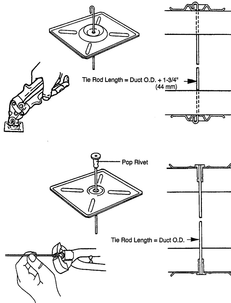
FIGURE 6-5-8 Terminations: Fasloop Pop Rivet Sleeve Locking Cap
