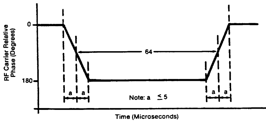
Figure 1.-DPSK Phase Characteristic
